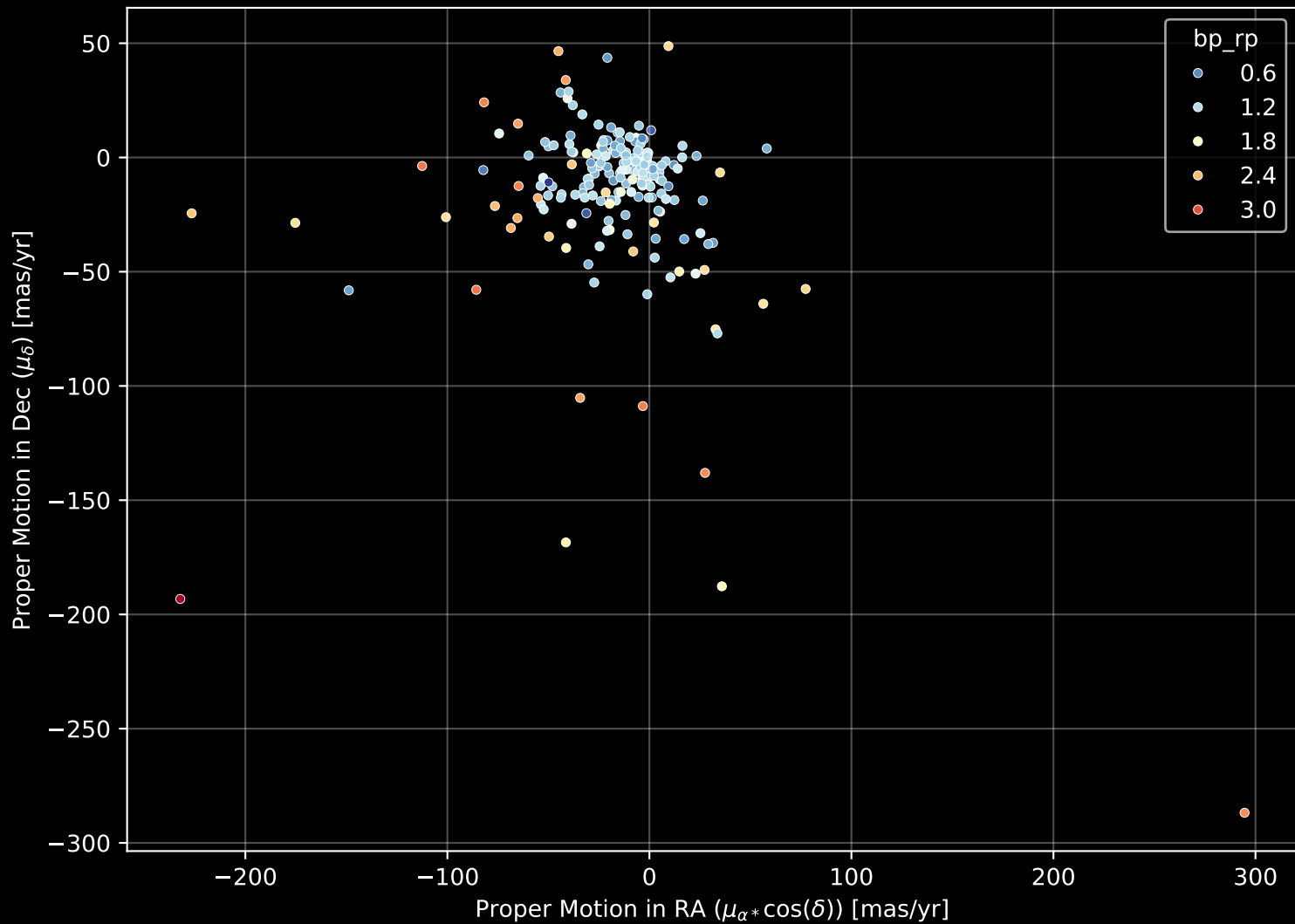
APOGEE DR17 Field: [K2_C14_237+51] Proper Motion Diagram (n= 209)
