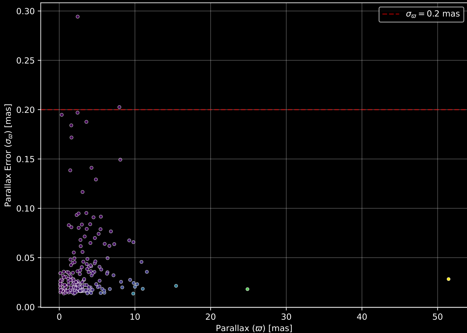
APOGEE DR17 Field: [K2_C14_237+51] Parallax Quality (n= 209)
