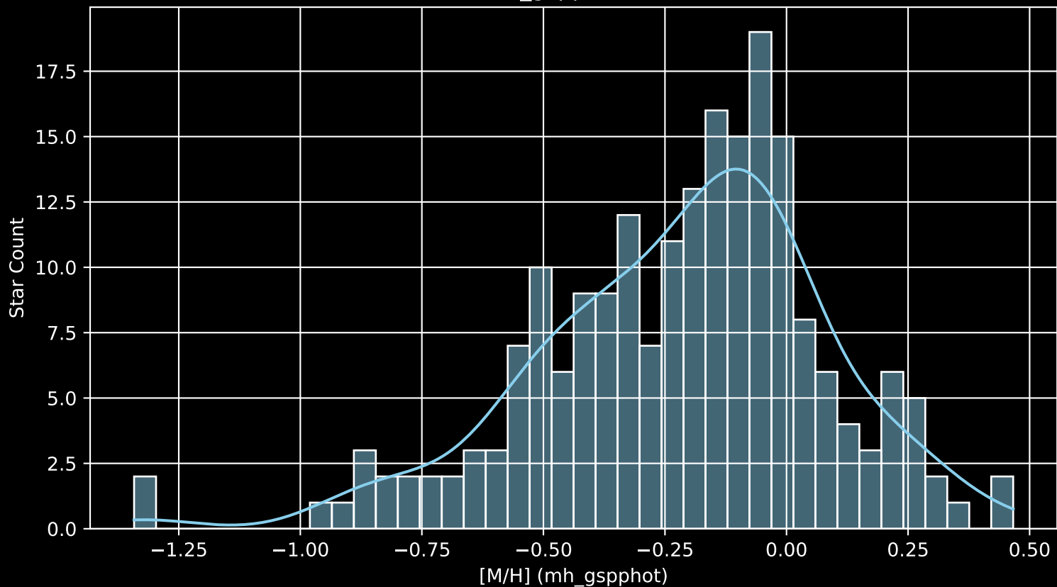
APOGEE DR17 Field: [K2_C14_237+51 [M/H] (mh_gspphot) (n= 207)
