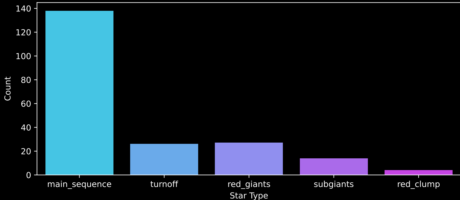
APOGEE DR17 Field: [K2_C14_237+51] Count plot of Star Type
