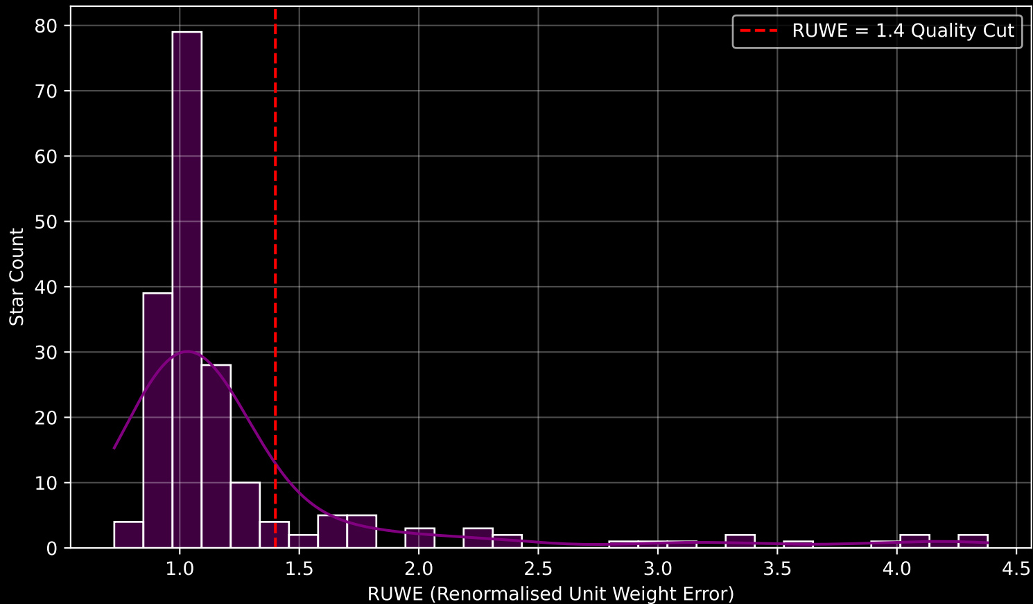
GAPOGEE DR17 Field [K2_C14_237+51] RUWE Distribution (n= 196)
