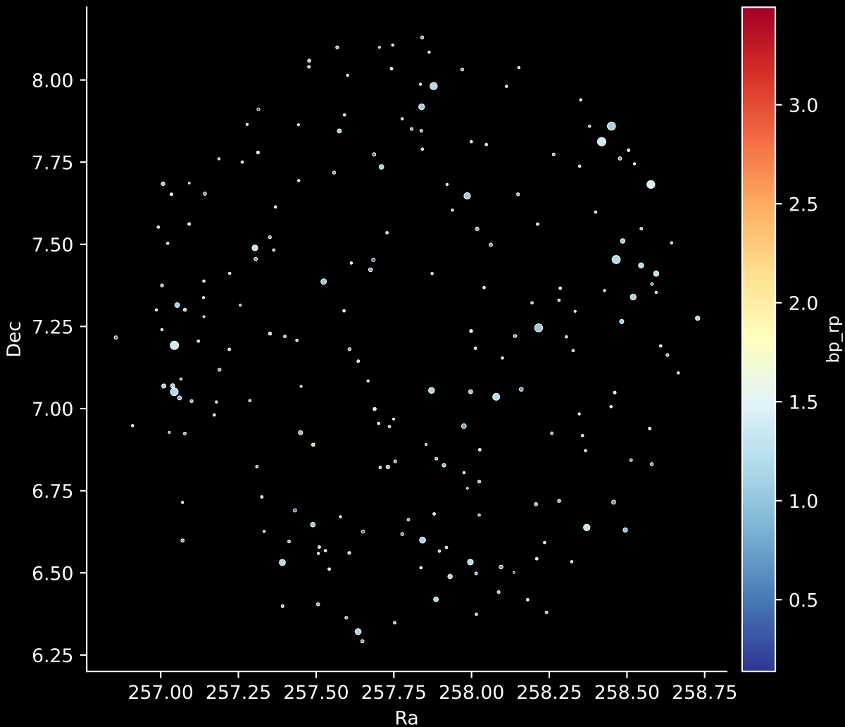
APOGEE DR17 Field: [K2_C14_237+51] Stars: 209
